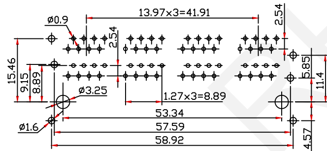
PCB Layout
